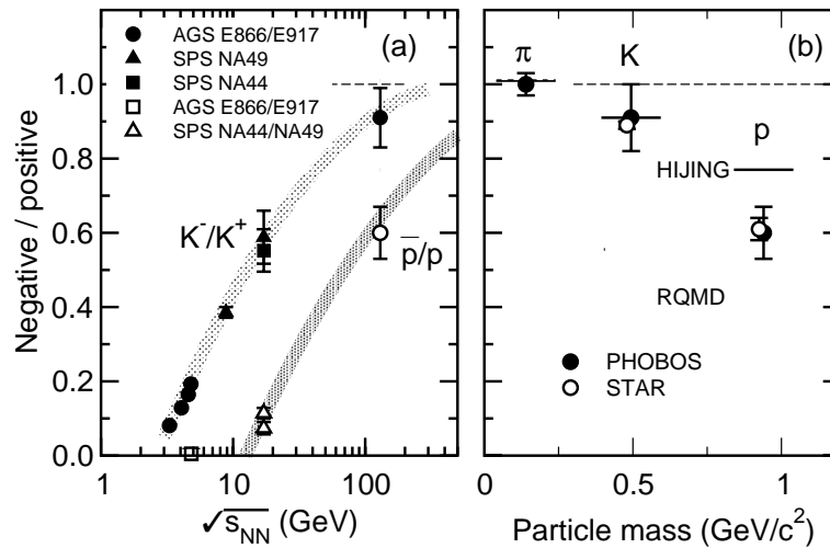
Figure 10. (a) K^-/K^+ and \bar{p}/p ratio shown as a function of energy [8,25,26]. The wide bands are drawn to guide the eye. (b) \pi^-/\pi^+ , K^-/K^+ and \bar{p}/p ratios for 130 GeV Au + Au collisions ( \bullet , PHOBOS [24]) and ( \circ , STAR [27]), compared to HIJING [16] (—) and RQMD [28] (- -) predictions.
