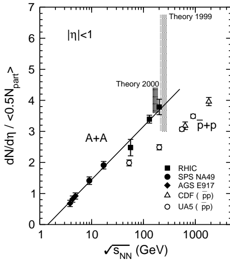
Figure 3. The scaled charged-particle density dN/d\eta / \langle \frac{1}{2} N_{\text{part}} \rangle for central Au + Au collisions at AGS [5], RHIC [6,7] and Pb + Pb collisions at the SPS [8] are shown as solid points as a function \sqrt{s_{NN}} . The \bar{p}p data from UA5 [9] and CDF [10] are shown as open symbols. The range of theoretical predictions for 200 GeV (light shaded band labeled Theory 1999) [11] are seen to be strongly reduced by the availability of the 130 GeV RHIC data.
