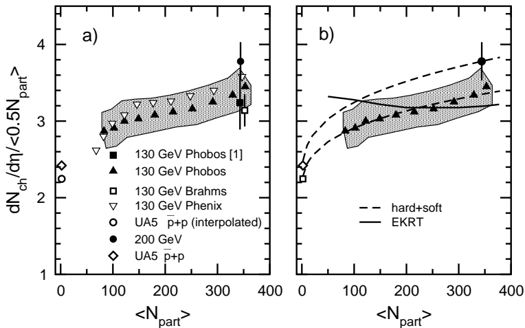
Figure 5. (a) Comparison of centrality dependence of dN/d\eta / \langle \frac{1}{2} N_{part} \rangle obtained by PHOBOS ( \blacktriangle ), PHENIX ( \triangle ) and BRAHMS ( \square ) at 130 GeV and PHOBOS at 200 GeV ( \bullet ). (b) Comparison to theoretical predictions (see text).
