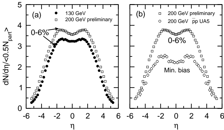
Figure 7. (a) Comparison of scaled charged-particle density distributions for 130 GeV ( \bullet ) and 200 GeV ( \square ) for the 0–6% centrality bin. (b) Comparison of the scaled charged-particle density distribution for central Au+Au ( \square ) and \bar{p}p ( \circ ) [9] collisions. Systematic errors of 7–10% are not shown for clarity.
