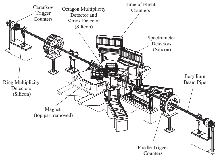
Figure 1. Schematic drawing of the PHOBOS setup. See text for details.
