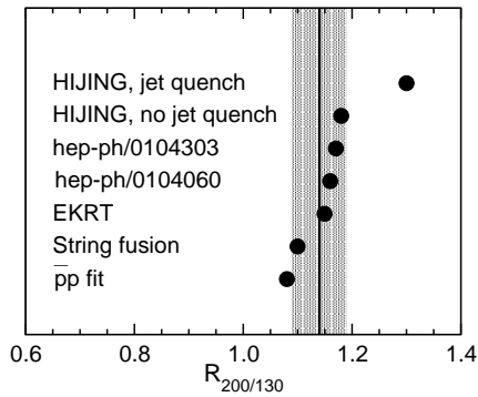
Figure 4. The measured increase in dN/d\eta / \langle \frac{1}{2} N_{\text{part}} \rangle with energy from 130 GeV to 200 GeV (shaded band) is compared with theoretical predictions [12–16] and a fit to \bar{p}p data [10]. The shaded band corresponds to the 90% confidence limit.
