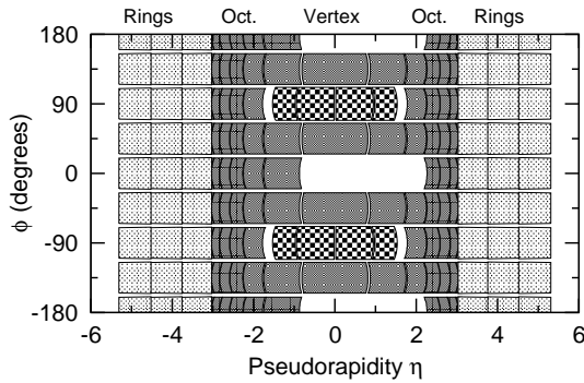
Figure 2. The geometrical acceptances of the ring (light), octagon (medium) and inner vertex (checker board) detectors for particles emitted from the nominal interaction point are shown as a function of \eta and azimuthal angle \phi .
