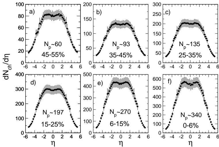
Figure 6. The charged-particle density distributions are shown for six centrality bins denoted by fraction of cross-section and mean number of participants, \langle N_{\text{part}} \rangle .
