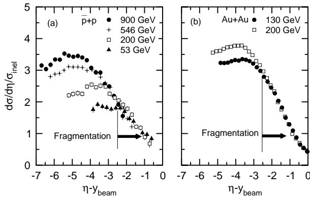
Figure 8. Illustration of scaling in the fragmentation region for \bar{p}p (a) and Au + Au (b) collisions.
