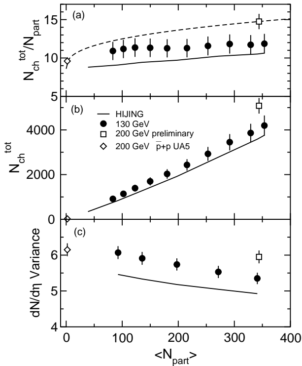
Figure 9. Centrality dependence of (a) the total charged-particle multiplicity per average number of participant \langle N_{\text{part}} \rangle , (b) the total charged-particle multiplicity, and (c) the variance of the dN/d\eta distributions ( -5.4 < \eta < 5.4 ) are compared to HIJING calculations (solid curves). See text for details.
