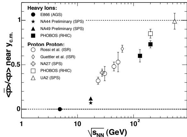
FIG. 2: Antiproton to proton ratio near midrapidity as a function of \sqrt{s_{\text{NN}}} for p+p collisions (open symbols) and central heavy ion collisions (filled symbols). The error bars represent the statistical and systematic errors in the measurements added in quadrature.
