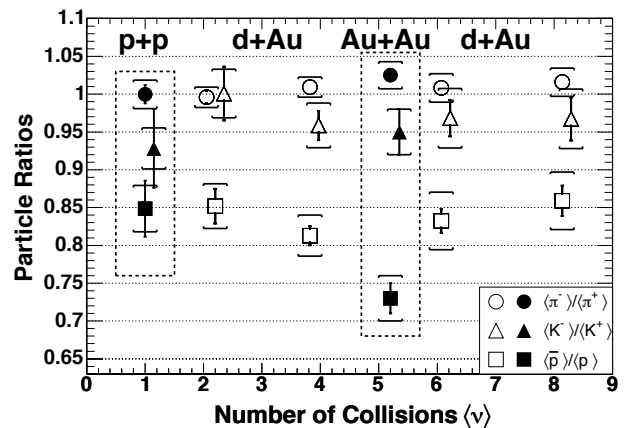
FIG. 1: Particle ratios as a function of centrality for each species for the p+p, d+Au and 12% most central Au+Au collision systems at \sqrt{s_{NN}} = 200 GeV. The brackets represent the total systematic error. The value of \langle \nu \rangle has been shifted by +0.15 for the measured \langle K^- / K^+ \rangle ratios for clarity.
