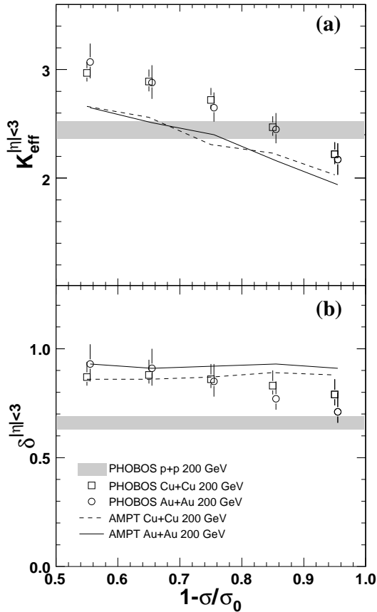
FIG. 4: (a) K_{\text{eff}} and (b) \delta as a function of fractional cross section for PHOBOS data (open symbols) and from the AMPT model (lines) in Cu+Cu (squares) and Au+Au (circles) collisions for |\eta| < 3 at \sqrt{s_{NN}} = 200 GeV. The error bars for data points represent systematic errors with 90% C.L. Results from p+p collisions at \sqrt{s} = 200 GeV [6] are shown by the shaded band.
