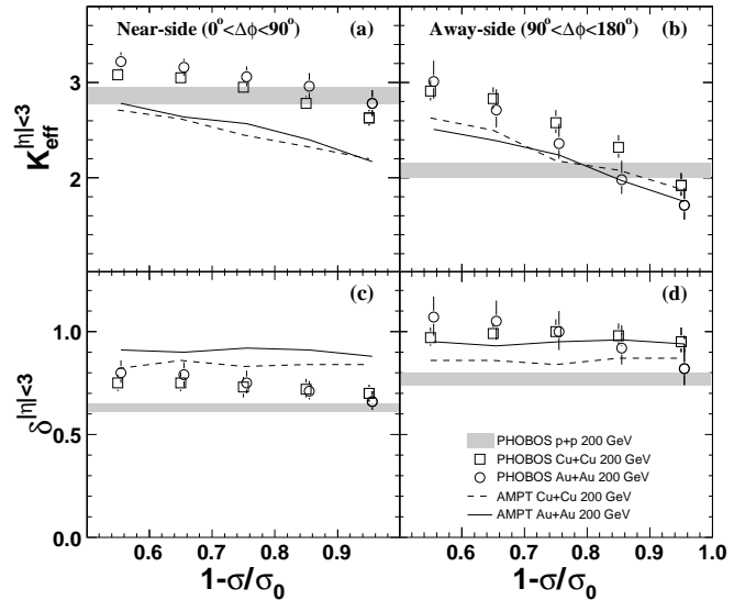
FIG. 5: Near-side (left column) and away-side (right column) K_{\text{eff}} (upper row) and \delta (lower row) as a function of fractional cross section for PHOBOS data (open symbols) and from the AMPT model (lines) in Cu+Cu (squares) and Au+Au (circles) collisions for |\eta| < 3 at \sqrt{s_{NN}} = 200 GeV. The error bars for data points represent systematic errors with 90% C.L. Results from p+p collisions at \sqrt{s} = 200 GeV [6] are shown by the shaded band.
