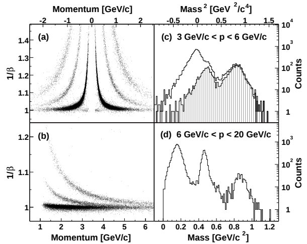
FIG. 1: Particle identification capability in BRAHMS. (a) and (b) Separation between pions, kaons, and protons. The MRS (a) is at 90^\circ and both charges are accepted. The FS (b) is here positioned at 12^\circ degrees. (c) Mass-squared spectrum in the FS from time-of-flight measurements. The shaded histogram includes the vetoing of pions in C1. (d) Mass spectrum in FS using the RICH.
