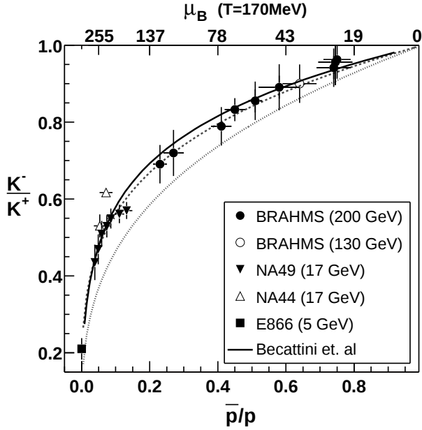
FIG. 4: Correlation between strange meson and baryon antiparticle-to-particle ratios. The NA44 and NA49 data are from Refs. [17] and [16], respectively. The E866 data are from Ref. [15]. The dashed line shows the relation K^-/K^+ = (\bar{p}/p)^{1/4} and the dotted line shows K^-/K^+ = (\bar{p}/p)^{1/3} . The full line shows the thermal prediction of Becattini et al.[18].
