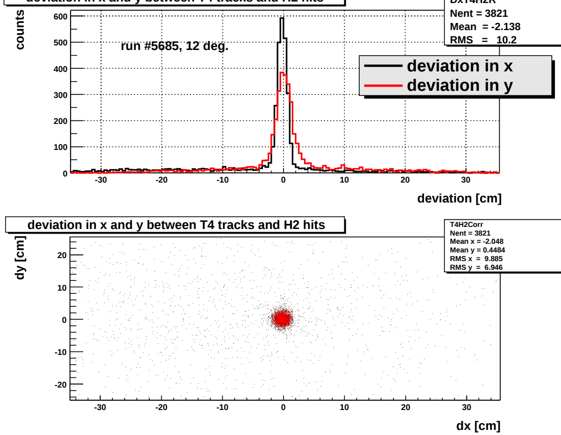
Figure 1: Black and red line histograms on the top panel correspond to correlation in x and y coordinate, respectively. Bottom panel shows the same correlation but in two dimensions, black color markers, and correlation for tracks that survive a \pm 2\sigma cuts both, for x and y coordinate, red color markers.
