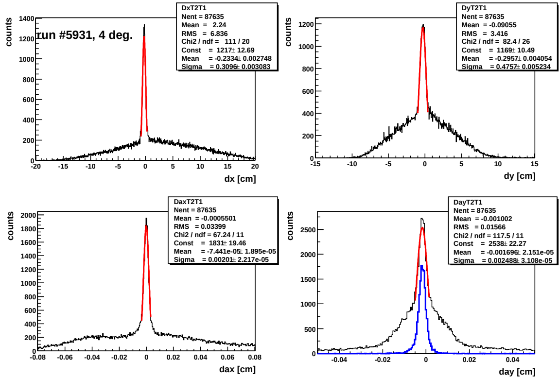
Figure 2: The correlation of the bfs (T2) and T1 tracks for the FS settings at 4 deg. Blue line histograms shows y-slope deviation distribution only for those tracks that match in x, y and x-slope (see also text).
