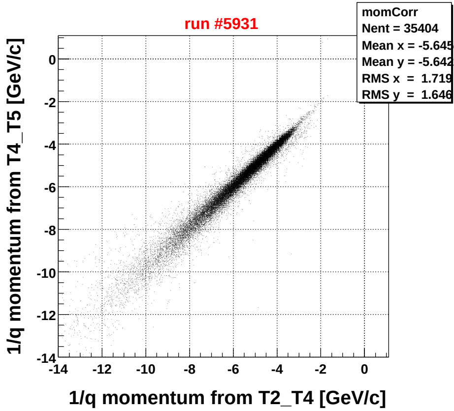
Figure 2: Correlation between momenta of the front (T2-D3-T4) and back (T4-D4-T5) section of each of the bfs track reconstructed in run 5931 (4 deg.)
