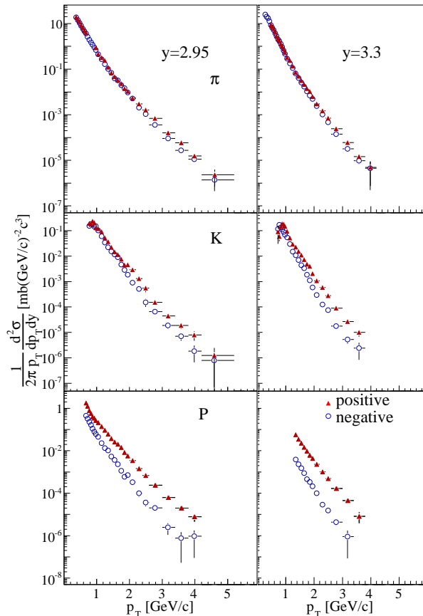
FIG. 1: Invariant cross section distributions for pion, kaons protons and anti-protons produced in p+p collisions at \sqrt{s} = 200 GeV at rapidities y=2.95 (left panels) and y = 3.3 (right panels). In all panels, positive charged particles are shown with filled triangles (red in online version) and negative ones with open circles (blue in online version). The errors displayed in these plots are statistical.
