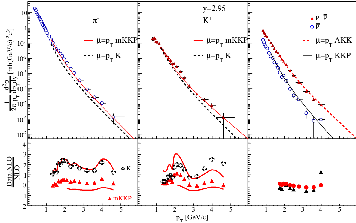
FIG. 3: Top) Comparison of invariant cross sections for \pi^- , K^+ , \bar{p} and the sum \bar{p} + p at y=2.95 and NLO calculations. The calculations were performed with factorization and renormalization scales both set to p_T . The mKKP set of fragmentation functions (full red line online) produce the best agreement with the \pi^- and K^+ data. The sum \bar{p} + p is well described by calculations that use the AKK set (dashed red line in online version) while the KKP describes the \bar{p} s (see text for details). Bottom) Relative differences between data and calculations. For the mesons the top smooth curve shows the effect of setting \mu = 2p_T and the bottom curve \mu = 1/2p_T . For the baryons the (red) filled circles are \bar{p} + p data vs the AKK set while the filled triangles are for \bar{p} s versus the KKP set.
