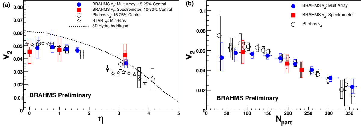
FIGURE 1. (a) Integrated v_2 versus \eta for charged hadrons. The BRAHMS spectrometer results are consistent, but systematic errors with the spectra may distort the shape. For comparison, a 3D hydro model results [11] are plotted. (b) Integrated v_2 versus N_{part} for charged hadrons within -1.0 < \eta < 1.0 .
