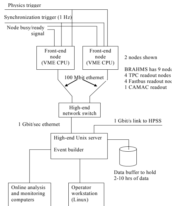
Figure 26 BRAHMS DAQ data flow.
