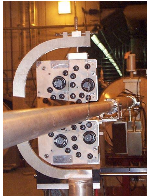
Figure 22. The beam-beam counter array. The left beam-beam counter array is shown at the top and the right array at the bottom. The C-shape holder in the picture is part of the beam pipe support system placed \sim 30 cm in front of the BBC array. The large and the small solid angle elements are clearly distinguishable in the photo.
