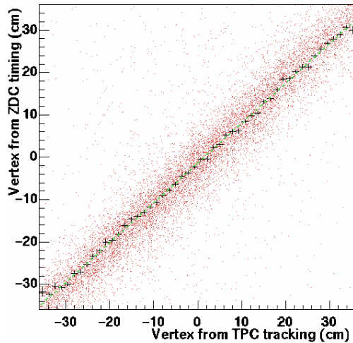
Figure 28 Correlation between vertex determination from the ZDCs and the TPM1 time projection chamber.
