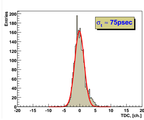
Figure 23 Time distribution between a start detector and one of big tube counters in a test beam set up at the AGS (see the text for further details).
