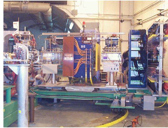
Figure 4. The Mid-Rapidity Spectrometer. TPM1 and TPM2 are visible on the left and right, respectively, of the magnet D5. The time of flight wall, TOFW, is visible on the far right. The nominal interaction vertex surrounded by the global detectors is visible on the far left.
