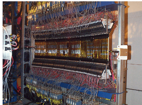
Figure 13. Mid-Rapidity Spectrometer Time of Flight wall.
