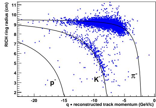
Figure 33 Preliminary PID obtained from the RICH detector. The lines indicate the theoretical positions of the particles in the plot.
