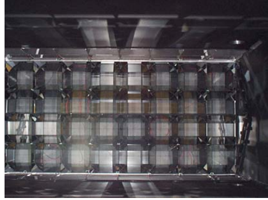
Figure 17. A photograph of the mirror system of C1. The picture was taken from the entrance window. The reflection of the array of light funnels (Winston cones), that direct the light onto the PMT arrays, is clearly visible.
