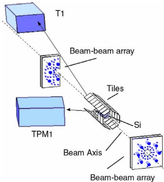
Figure 19. Schematic depiction of the multiplicity array and beam-beam counters relative to other parts of the spectrometer. Recall that a photograph of the global detectors is shown in Figure 5.
