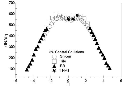
Figure 29. Pseudo-rapidity distributions from 5% central Au+Au collisions at 130 GeV/u center of mass energy measured with the multiplicity array, beam-beam counters and TPM1. The results from the tiles (open squares) are systematically higher than the Si strip data (open circles) in the mid-rapidity range, a feature that is not understood quantitatively. The results from TPM1 (stars) agree quite nicely with the tile and Si at the same \eta .
