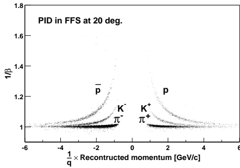
Figure 31. Time-of-Flight versus track momentum for charged particles tracked through D2 in the FFS. The TOF was measured by H1. Data for positive and negative charge are from runs with different magnet polarities added together to make one spectrum.
