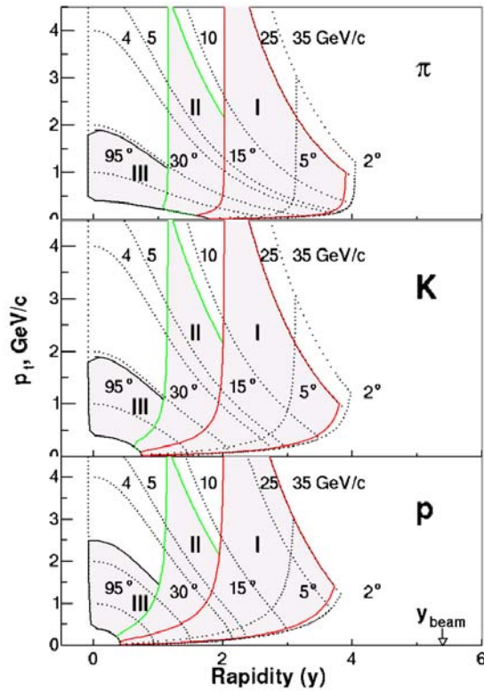
Figure 1. BRAHMS Acceptance for pions, kaons and protons. Region I and II show the acceptance of the forward spectrometer with two different configurations, see below. Region III shows the acceptance for the Mid-Rapidity Spectrometer. The dotted curves marked 4, 5, 10, 25 and 35 GeV/c are curves of constant momentum, while the set marked 95, 30, 15, 5, 2 degrees indicate curves at constant polar angle. The fully drawn curves mark the acceptance borders.
