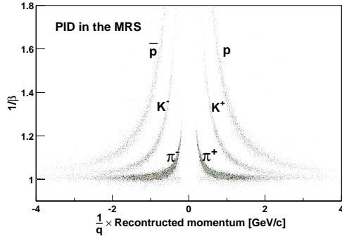
Figure 30. Time of flight of charged particles in TOFW as a function of reconstructed particle momentum obtained from tracking in TPM1 and TPM2 through the D5 magnet.
