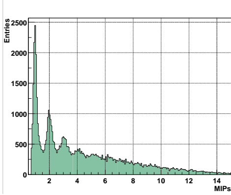
Figure 24 Normalized beam-beam counter ADC spectrum for minimum bias Au-Au collisions obtained with a 2 inch tube.
