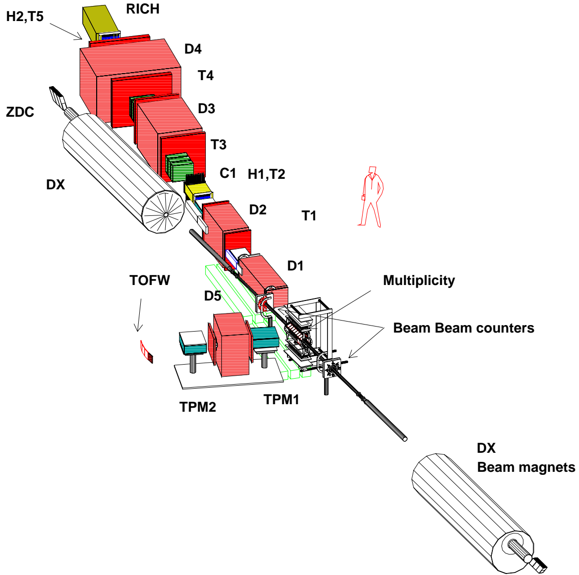
Figure 2. The BRAHMS detectors in perspective. The spectrometer magnets are denoted D1 through D5, the time of flight hodoscopes in FS are H1 and H2, and the tracking counters T1-T5, where T1 and T2 are time projection chambers and T3, T4 and T5 are multi-wire drift chambers. The two Čerenkov counters in FS are C1 and RICH. The tracking chambers of the MRS are TPM1 and TPM2, while the time of flight system is the TOFW. The global detectors are denoted as Beam-Beam counters and Multiplicity. The ZDCs are situated beyond the DX beam magnets. The distance between the front of the two DX beam magnets is 18m.
