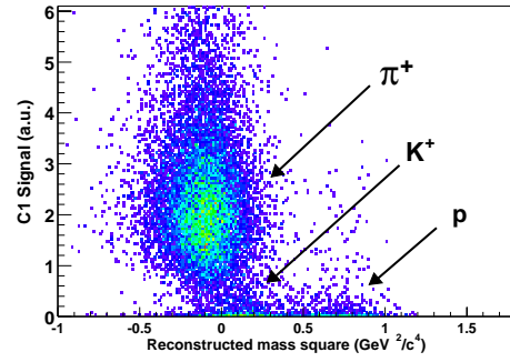
Figure 32. C1 preliminary normalized PMT response vs mass squared.
