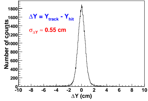
Figure 15. Number of tracks in H1 plotted against the difference in the y position of the extrapolated T2 track intersection with the slat, and the y position in H1 calculated by the time difference (top - bottom) for all reconstructed tracks hitting the slat.
