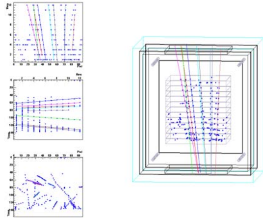
Figure 27. Online event viewed with the TPC 3d viewer (see the text for further explanation). The top left panel has the x-axis as the pad number and the y-axis as the row number (ie a projection of of the tracks onto x-z). The middle left panel has the x-axis as the row number and the y axis as the time (ie a projection of the tracks onto y-z). The bottom left panel shows a projection of the tracks onto x-y, the pad number on the x-axis and the time on the y-axis. Finally the right panel shows the 3D image of the tracks which is rotatable.
