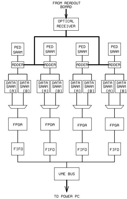
Figure 25. Schematic diagram for the TPC VME receiver board. The components described further in the text are the pedestal and data SRAM, the FPGA and the FIFO.
