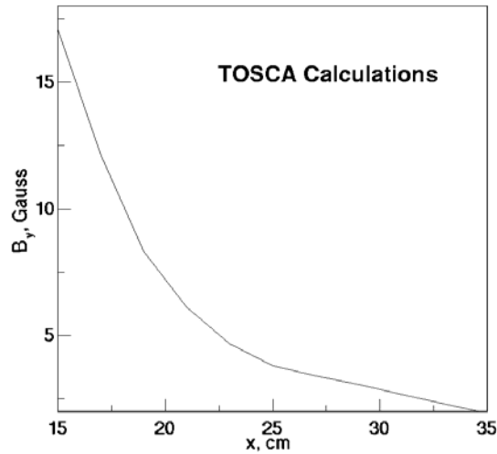
Figure 6. TOSCA calculations showing the fringe fields in the y-direction as a function of the distance from the center of D1. The beam is at x=23 cm when D1 is at 2.3 degrees.
