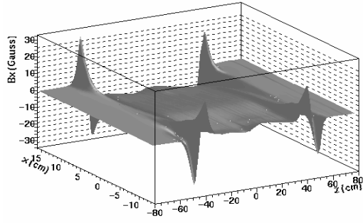
Figure 7. D5 B_x component measured 1 cm above the medium plane ( y=1 cm). The measurements were made with an average field of half the maximum value.
