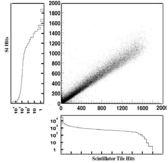
Figure 21. Particle multiplicity distributions for the Si strip detectors and scintillator tiles. The multiplicity distribution measured by the Si strip detector is shown to the left in the figure and the corresponding scintillator tiles measurement at the bottom. The correlation of the two measurements is shown as the scatter plot in the middle.
