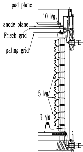
Figure 9. Design of the field cage and resistor chain. The cathode plane is at the bottom of the figure and is held at -5000 V, while the anode plane, near the top, is at ground potential. See the text for further details.
