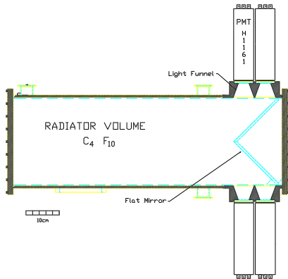
Figure 16 Schematic side view of the Čerenkov detector C1. For details, see the text.
