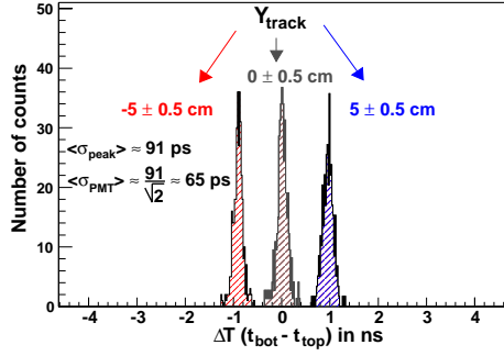
Figure 14. Time difference between top and bottom in a typical H1 slat. Tracks are required to intersect one of three 1cm regions along the length of the slat (y-direction).
