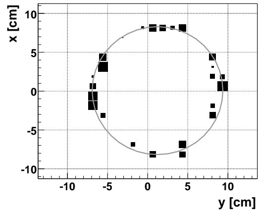
Figure 18 An event with a ring detected in the RICH detector.
