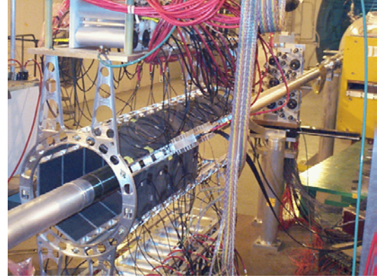
Figure 5. Global detectors. The photo shows the hexagonal barrel arrangement of the plastic tiles (dark square surfaces), the beam line and to the right, just in front of the yellow yoke of the D1 magnet, one of the beam-beam counter arrays, where the radiators show as dark circles. The Si strip detectors have been removed for the picture and the other beam-beam counter array is outside the photo to the left.
