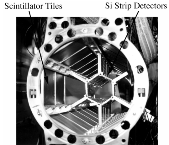
Figure 20 Multiplicity Array with the Si strip and the scintillator tiles detectors. The beam pipe is not seen.
