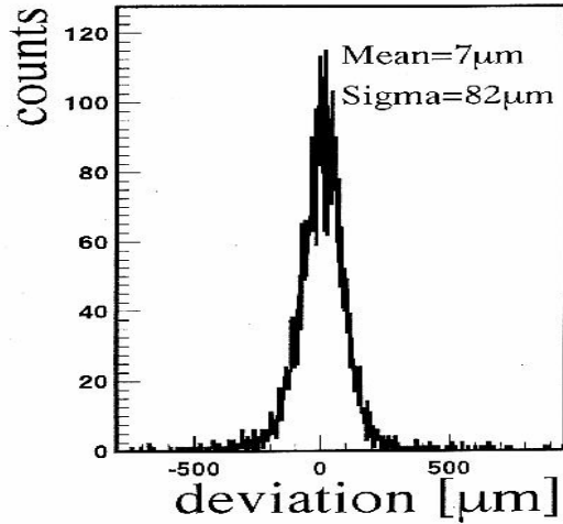
Figure 11. One particle position resolution of the T3 prototype detector measured during a test run.
