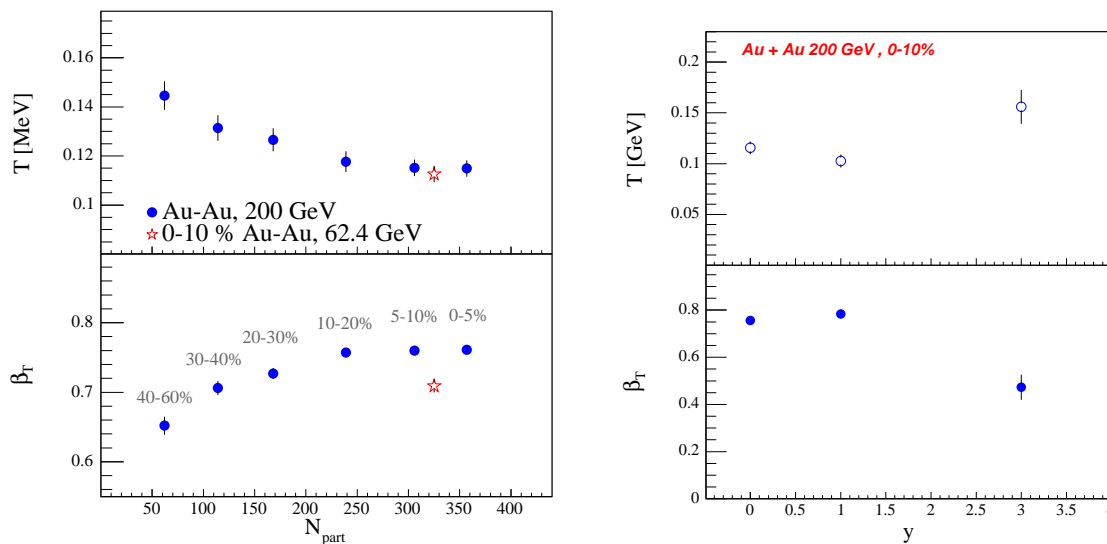
Figure 1: Kinetic freeze-out temperature and surface transverse flow velocity for AuAu collisions [9]. Left: Centrality dependence at y=0 ; Right: Rapidity dependence for central collisions.
