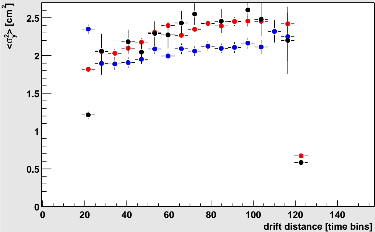
T2: Squared cluster width in time direction vs. drift distance
