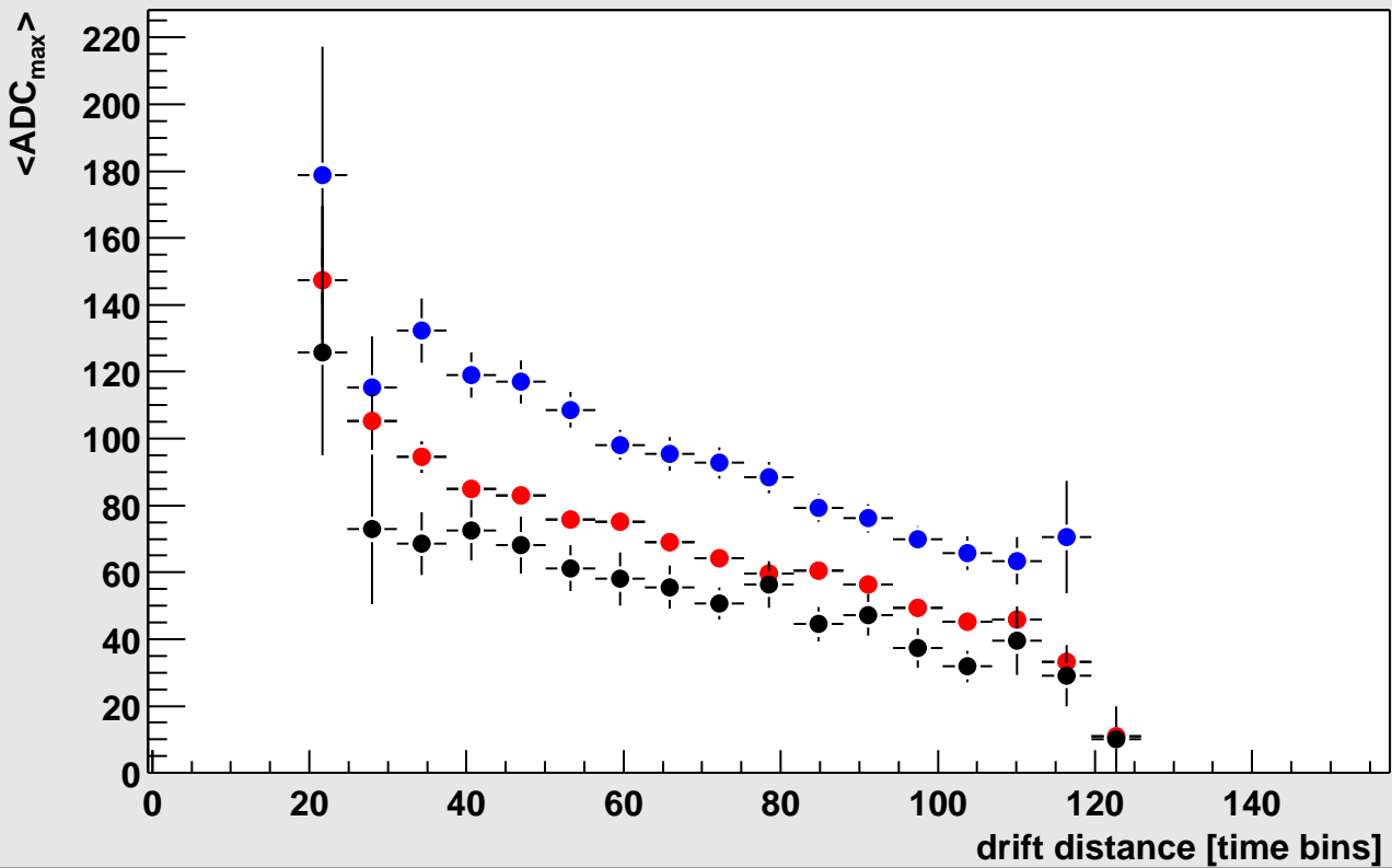
T2: Cluster max ADC vs. drift distance
