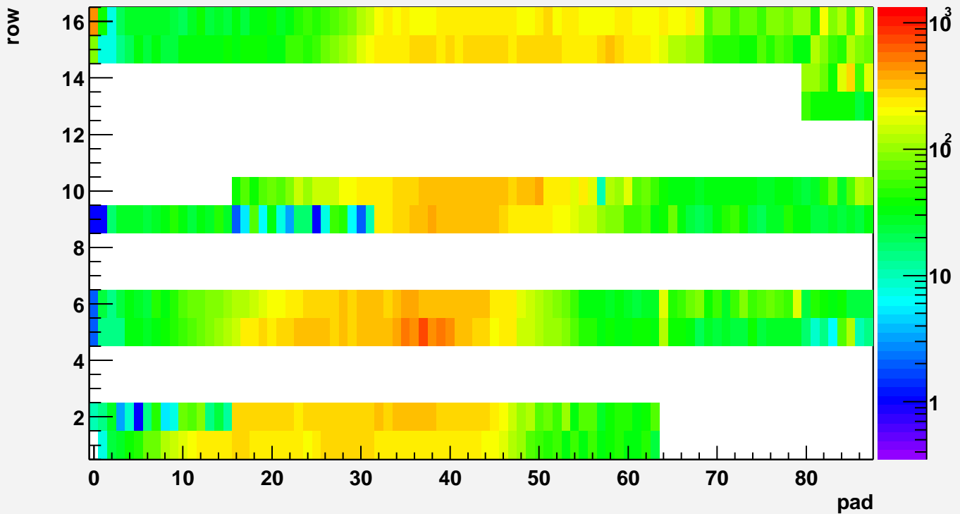
Pad efficiency T2
