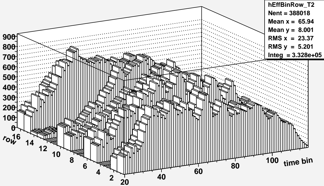
Time bin efficiency T2
