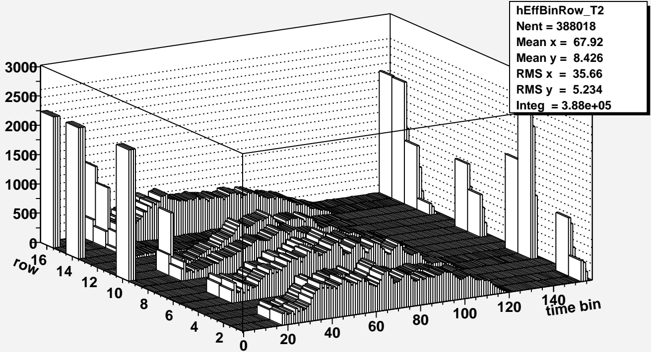
Time bin efficiency T2
