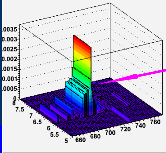
Pi0 Hits in X-strips (ShowerMax)
