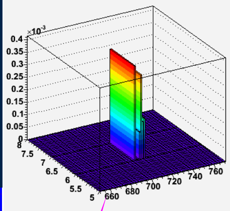
Pi0 Hits in X-strips (PreShower)
