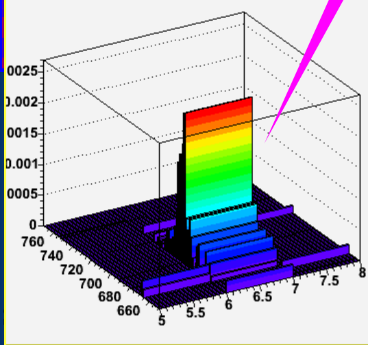
Pi0 Hits in Y-strips (ShowerMax)
